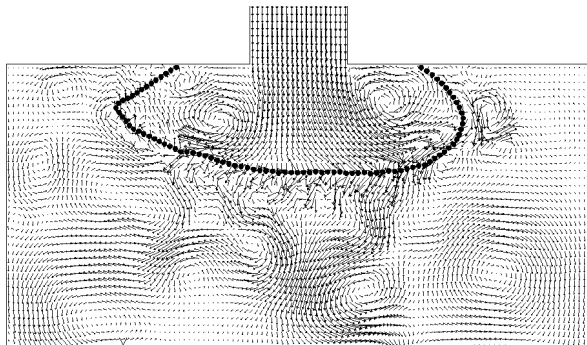
Figure 7: Instantaneous configuration for the elastic bag
