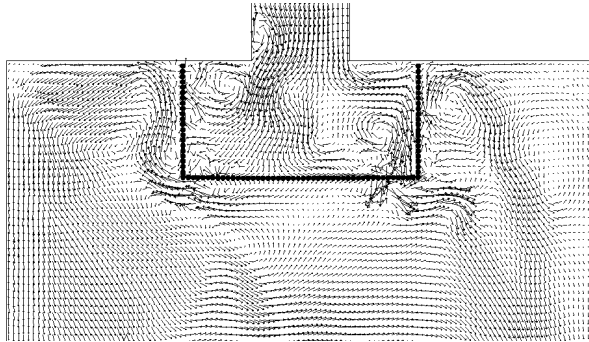
Figure 4: Flow configuration of the rectangular rigid bag
