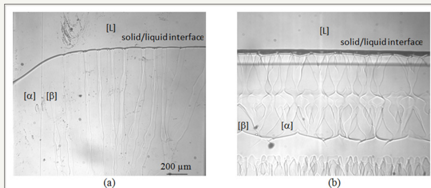
Figure 1: Isothermal peritectic coupled growth observed by using a glass sample with an inner width of 100µm (a) and one with an inner width of 600µm (b). The difference is obvious.
