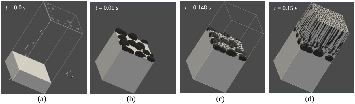
Figure 9: Formation of the binary and ternary eutectic. (a) surface section of the preexisting zinc phase, (b) nucleation of the Al phase at the zinc surface, (c) nucleation event of the \text{MgZn}_2 phase, and the solidification pattern of the ternary eutectic.
