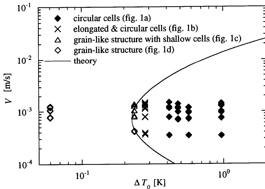
Fig. 2. For G_L = 5 \times 10^4 K/m and D = 6 \times 10^{-10} m 2 /s the neutral stability curve correlated best with the experimental observations. Note that the measuring error was \pm 40 mK for small \Delta T_0 and \pm 70 mK for the larger ones. The measuring error for V was less than \pm 0.07 mm/s.
