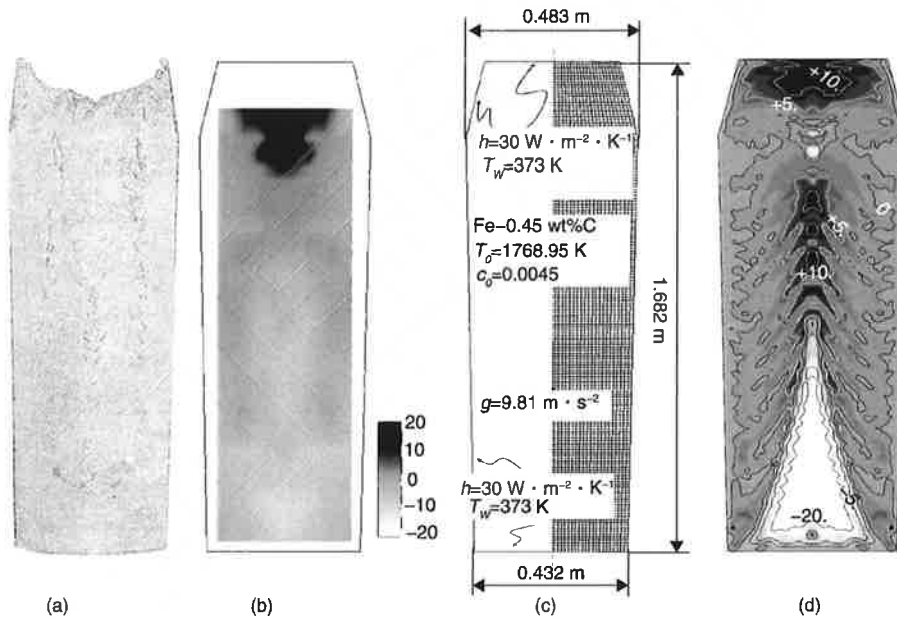
Fig. 6 Configuration of a 2.45-ton industry-scale steel ingot: (a) experimental ingot and (b) experimentally measured segregation [1] , (c) simulation settings and (d) simulated macrosegregation in grey scale (black for the positive segregation and light for the negative segregation) overlapped with isolines. The macrosegregation, both experimental (b) and simulated (d), is shown for the segregation index ( 100 \times (c_{\text{mix}} - c_o)/c_o ). Nucleation parameters for equiaxed crystals: n_{\text{max}} = 5 \times 10^9 \text{ m}^{-3} , \Delta T_o = 2 \text{ K} , \Delta T_N = 5 \text{ K}
