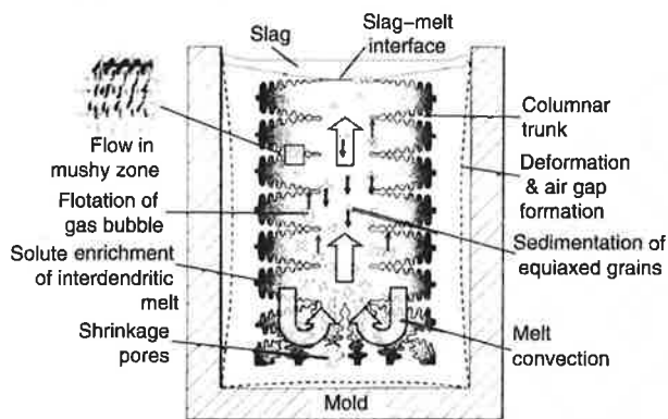
Fig. 1 Schematic illustration of the multiphase phenomena during solidification of a metal casting
