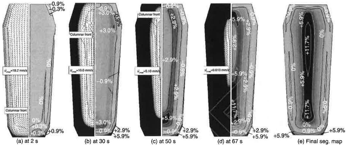
Fig. 2 Predicted solidification sequence and macrosegregation formation induced by thermosolutal convection in a benchmark ingot ( \phi 66 \text{ mm} \times 170 \text{ mm} ) of Fe-0.34 wt% C: the left half parts of figure 2a ~ d show the volume fraction evolution of the columnar phase in gray scale with the columnar tip position indicated with a solid line, vectors show the liquid velocity; the right half parts of the series show the evolution of the macrosegregation, gray-scaled according to positive and negative segregation, the macrosegregation index in % is calculated as 100 \times (c_{\text{mix}} - c_0)/c_0 , where c_{\text{mix}} is the liquid-solid mixture concentration. The predicted final macrosegregation map is shown in (e).
