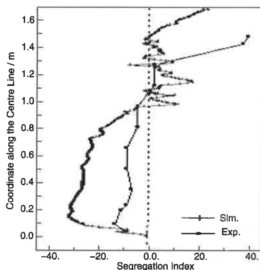
Fig. 8 Comparison of the numerically predicted macrosegregation ( 100 \times (c_{\text{mix}} - c_0)/c_0 ) along the ingot centreline with the experiment [1] . Nucleation parameters for equiaxed: n_{\text{max}} = 5 \times 10^9 \text{ m}^{-3} , \Delta T_{\sigma} = 2 \text{ K} , \Delta T_N = 5 \text{ K}
